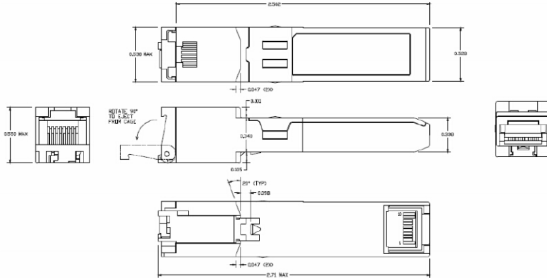
Figure2. Mechanical Specifications
