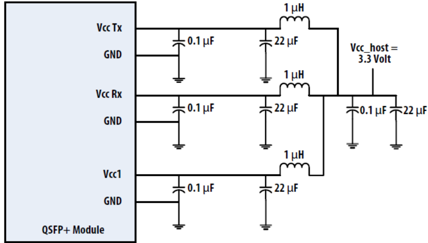
Figure2. Recommended Power Supply Filter
