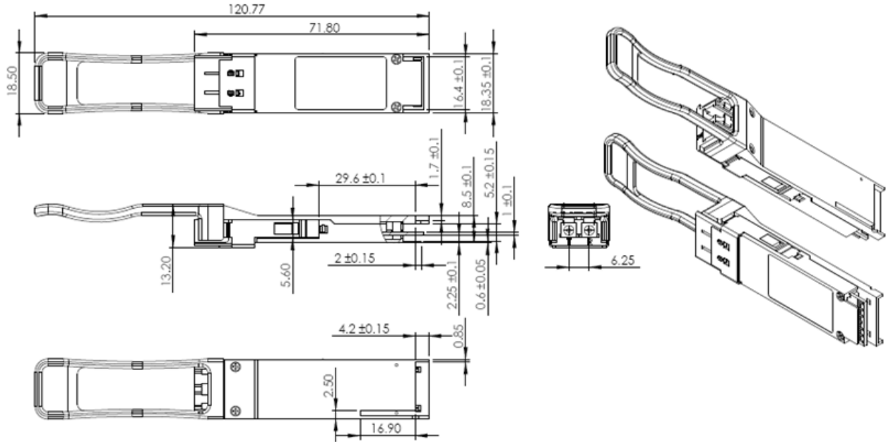
Figure3. Mechanical Specifications
