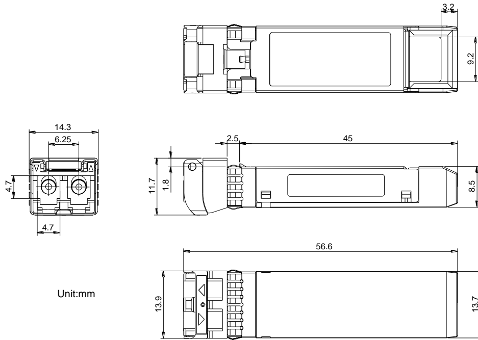
Figure4. Mechanical Specifications
